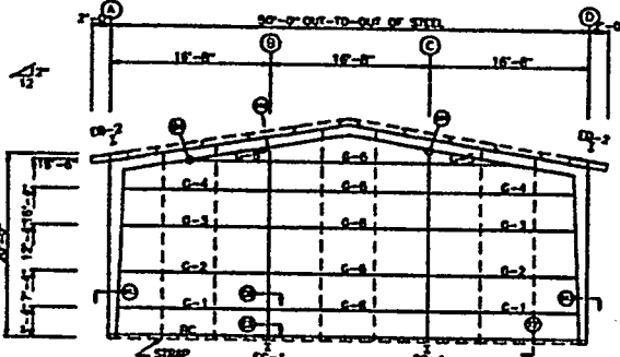
ENDWALL FRAMING: FRAME LINE 1
